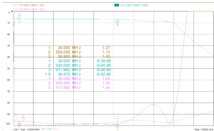
< Insertion Loss / Return Loss measurement >
